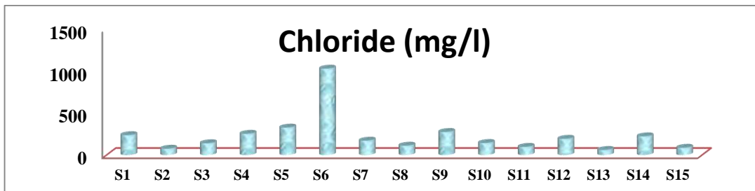
(Fig 4) Average distribution of Chloride in the sampling stations of Vilavancode Taluk
