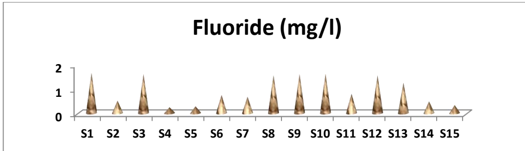
(Fig 2) Average distribution of Fluoride in the sampling stations of Vilavancode Taluk
