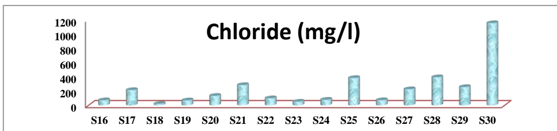
(Fig 4) Average distribution of Chloride in the sampling stations of Vilavancode Taluk
